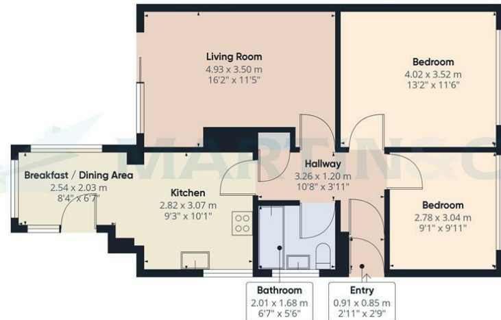
Floor 0 Building 1
