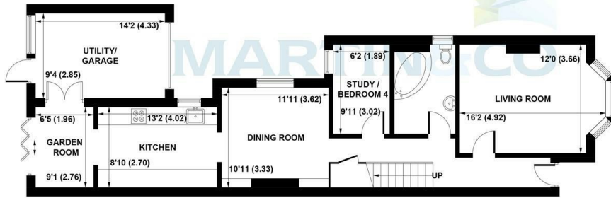
GROUND FLOOR
