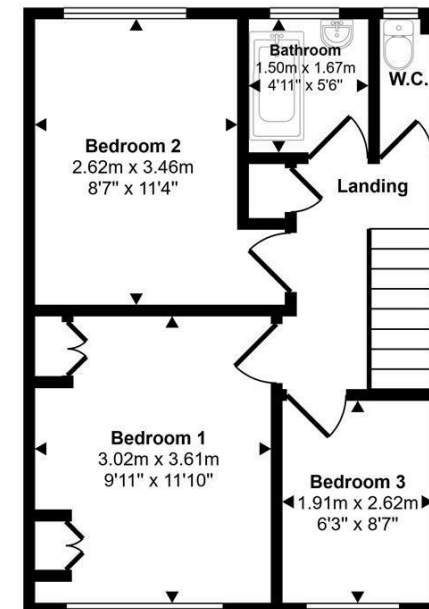
First Floor Approx 37 sq m / 402 sq ft
