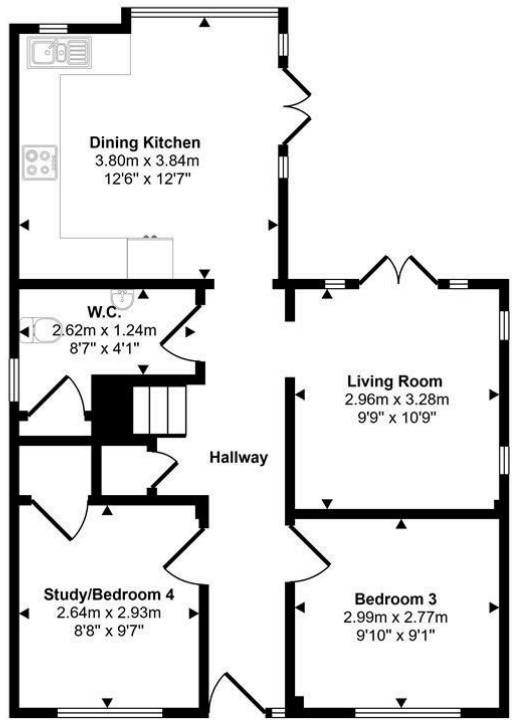
Ground Floor Approx 58 sq m / 625 sq ft
