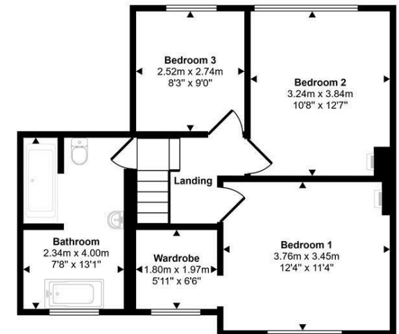
First Floor Approx 53 sq m / 567 sq ft
