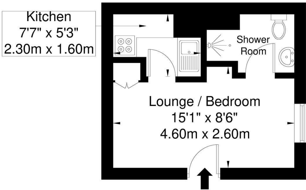
GROUND FLOOR 18.3 sq m / 196 sq ft
