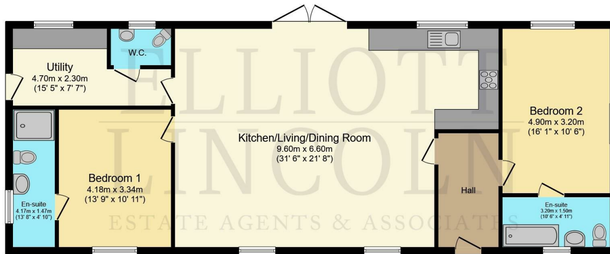
Floor Plan
