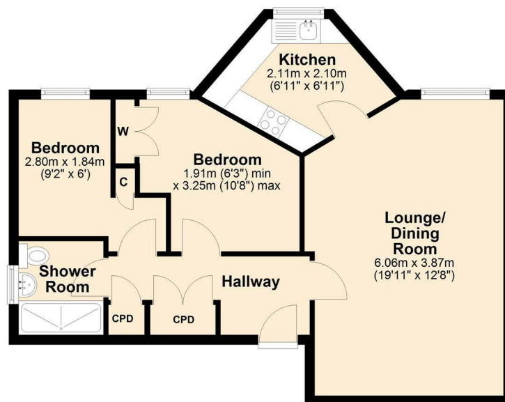
Third Floor
