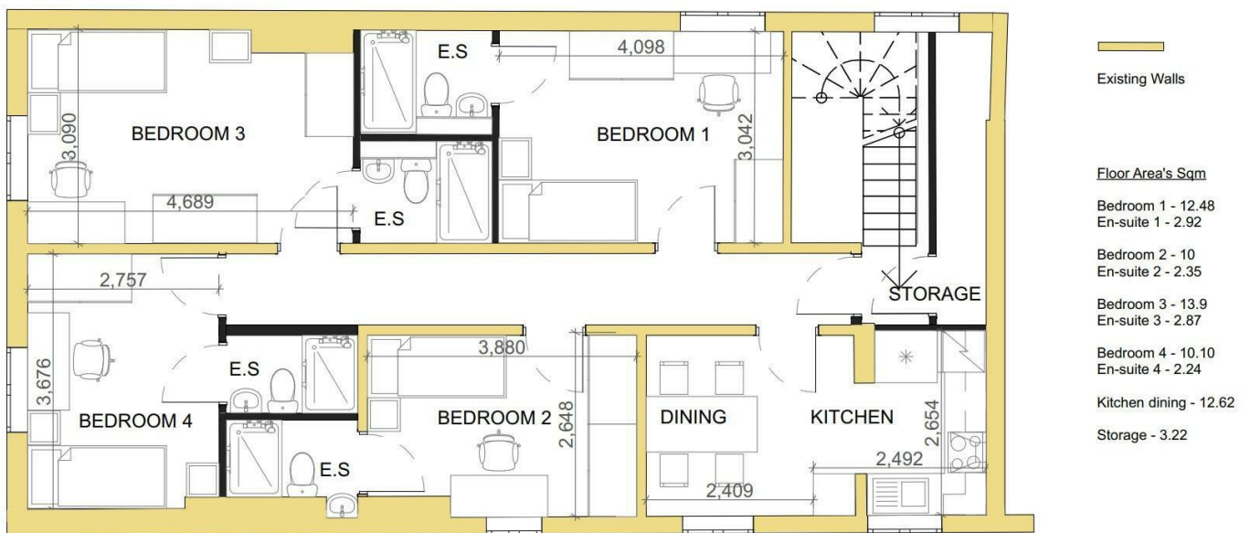
1:50 Proposed First Floor Plan
