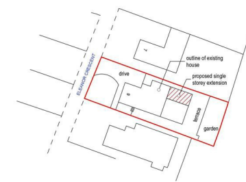
block plan
