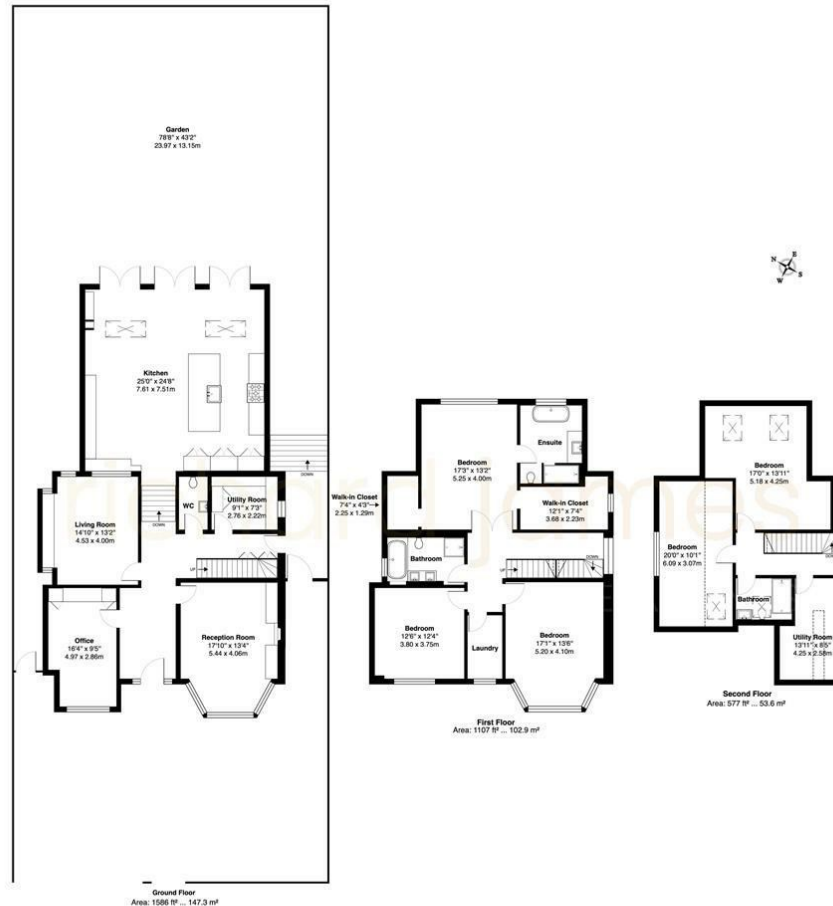
Parkside NW7 Total Gross Area 3382 sq ft ... 314.2 sq m Floor plans are for identification and guidance purposes only, not to scale. Complete NPS scale of measuring parameters.
