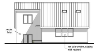
proposed front (west) elevation
