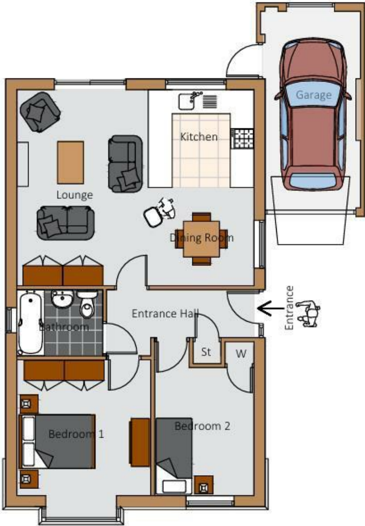
5 GROUND FLOOR scale nts
