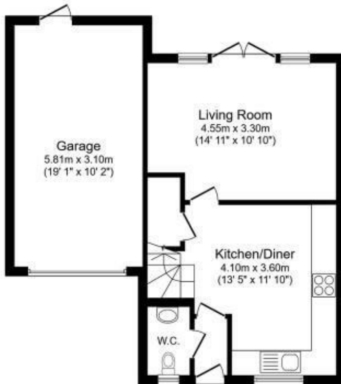
Ground Floor Floor area 52.6 sq.m. (566 sq.ft.)
