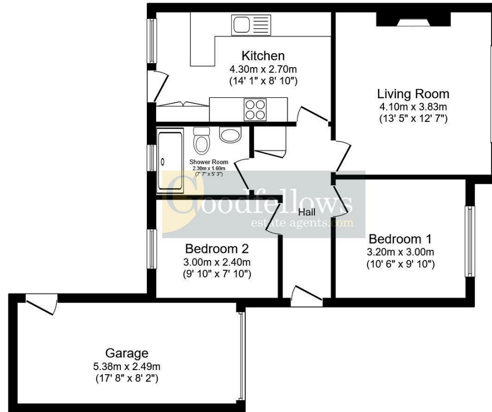
Floor Plan
