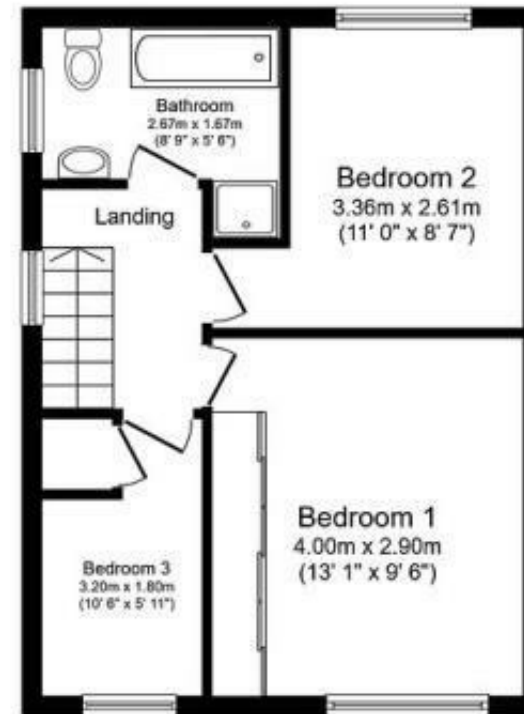
First Floor Floor area 40.1 sq.m. (432 sq.ft.)
