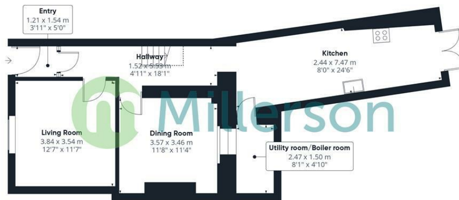
Floor 0 Building 1
