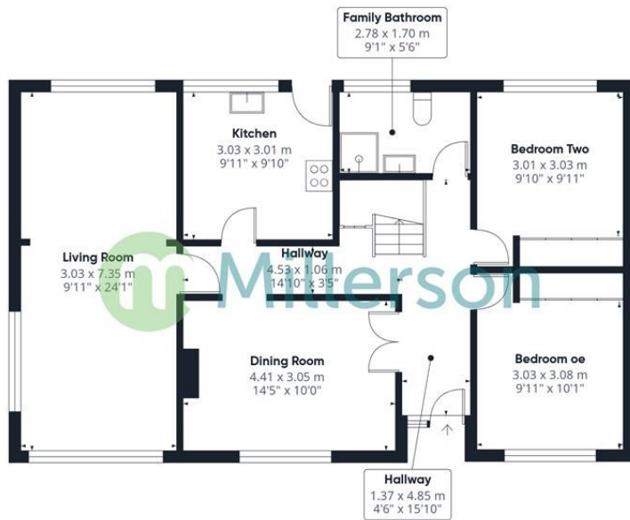
Floor 0 Building 1
